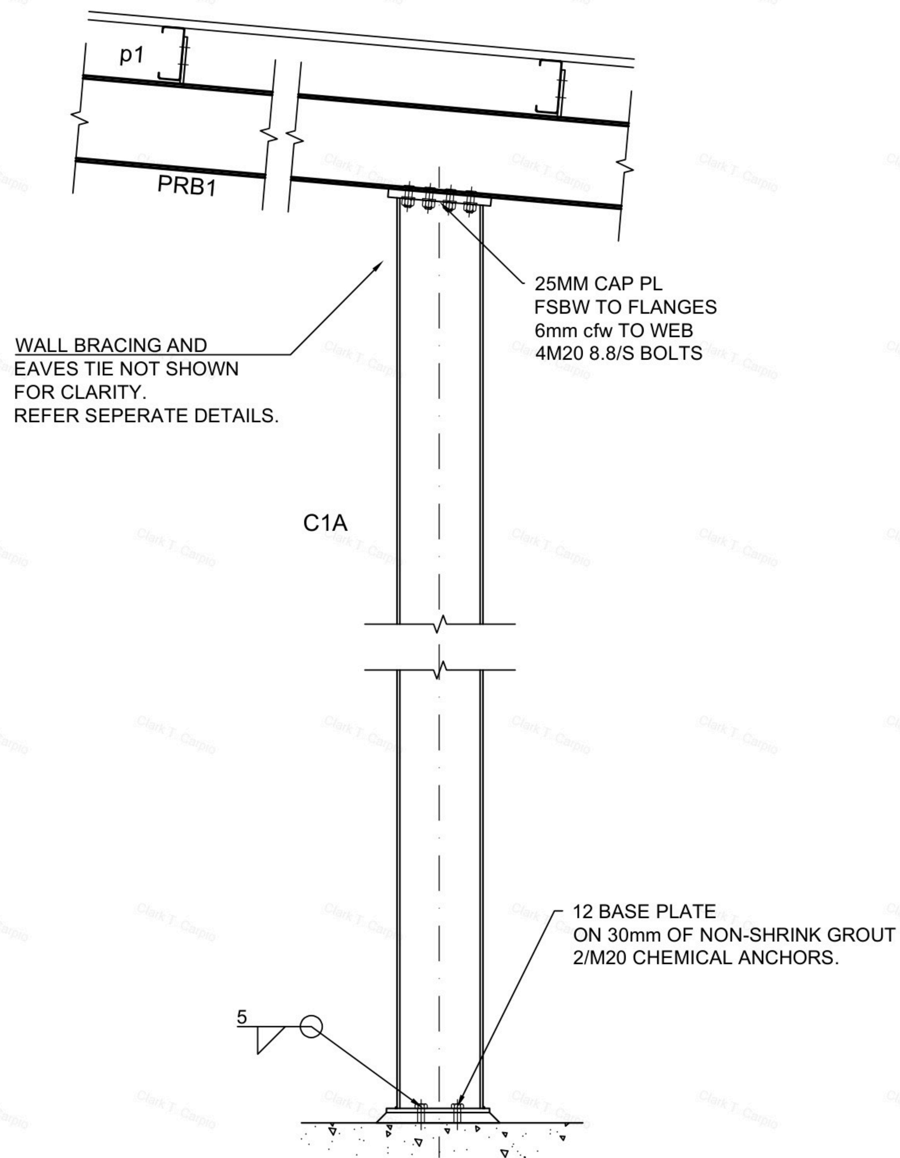
TYPICAL COLUMN CAP & BASE DETAIL
