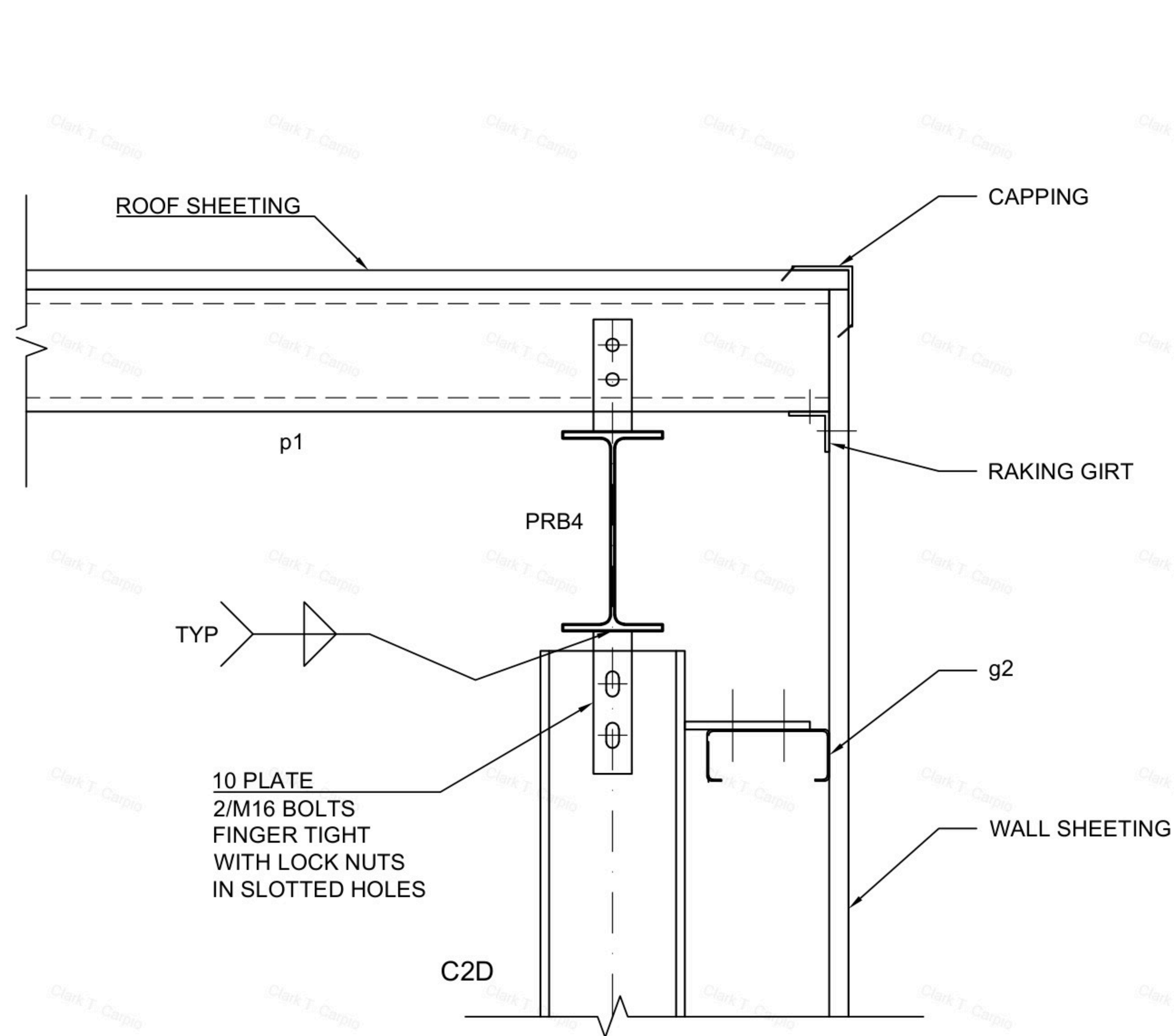
DETAIL C2D / PRB4
